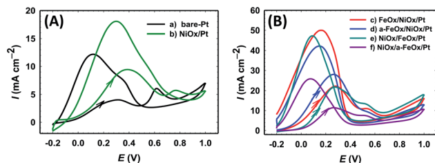
Fig. 5 CVs of the FAOR for the (a) bare-Pt, (b) NiOx/Pt, (c) FeOx/NiOx/Pt, (d) a-FeOx/NiOx/Pt, (e) NiOx/FeOx/Pt and (f) NiOx/a-FeOx/Pt electrodes in 0.3 mol L -1 FA (pH 3.5).
