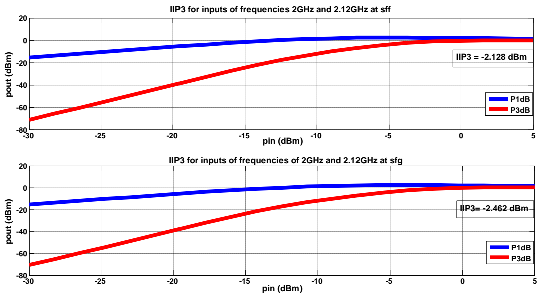
Fig. 5.32 Out-of-band IIP3 for two inputs of 2.1GHz and 2.12GHz at sff and sfsg
