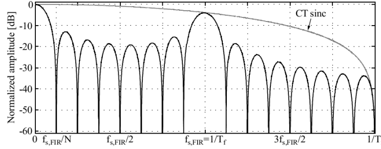
Fig. 3.7 FIR charge sampling sinc filter response
