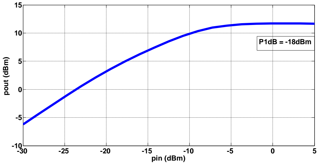
Fig. 5.14In-band P1dB for input signal of frequency 501MHz
