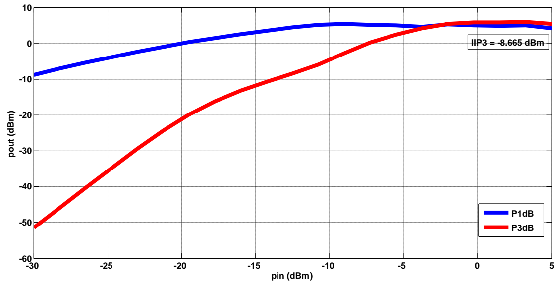
Fig.6.21 In-band IIP3 for input frequencies of 1.001GHz and 1.003 GHz with switches and matching network post layout
