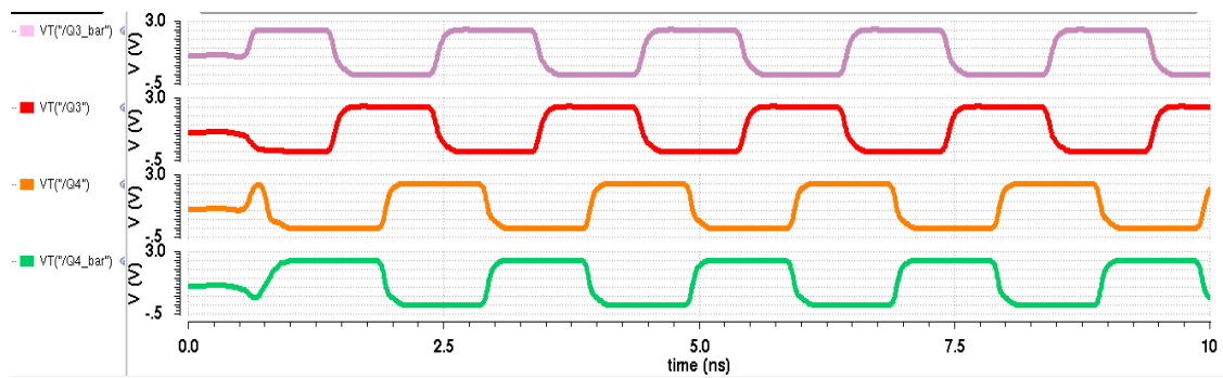
Fig. 4.16 Quadrature 50% duty-cycle Q3,Q3_bar,Q4 and Q4_bar
