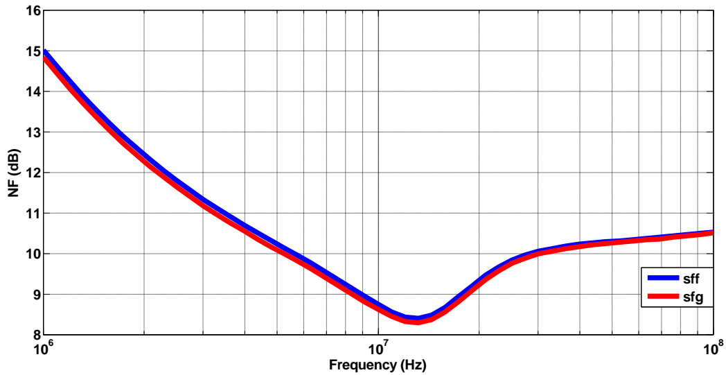
Fig. 5.25 NF at 2GHz at sff and sfg
