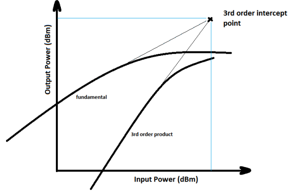
Fig. 2.2 IIP3 curve
