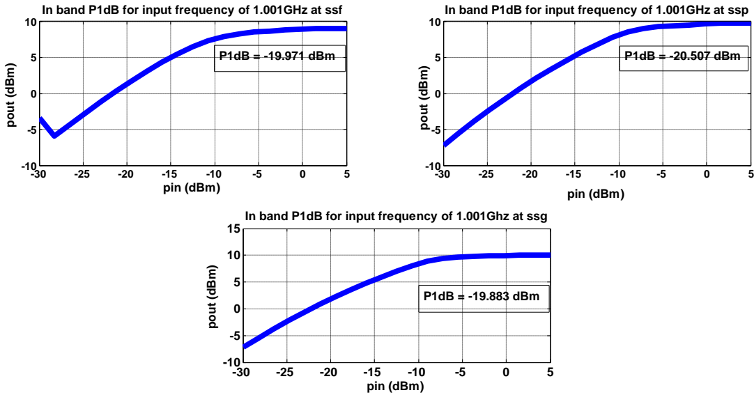
Fig.5.63 In band P1dB for input frequency of 1.001GHz at ssf, ssp and ssg
