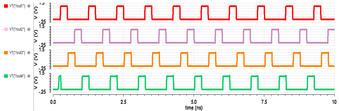
Fig. 4.24Non-overlapping 25% duty-cycle clocks ( out1\_MN , out2\_MN , out3\_MN and out4\_MN )
