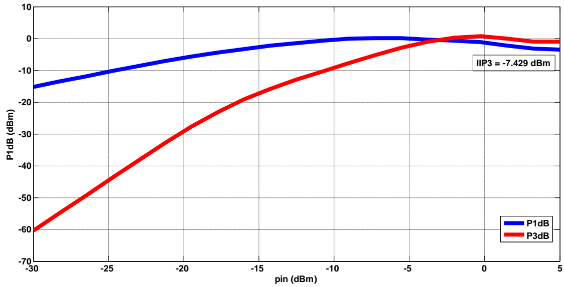
Fig.6.20 Out-of-band IIP3 for input frequencies of 1.1GHz and 1.12GHz with switches and MN post layout
