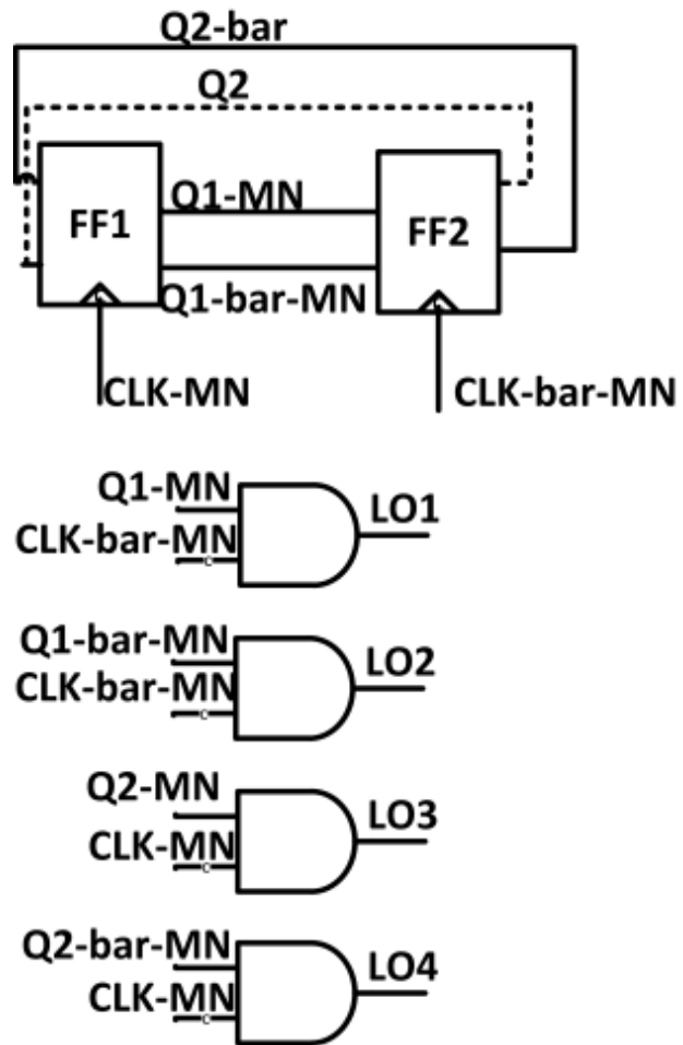
Fig. 4.25 The digital circuitry generating the MN controlling clocks
