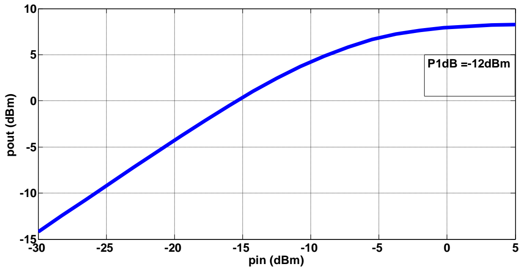
Fig. 5.4 Out-of-band P1dB for input signal of 2.1GHz
