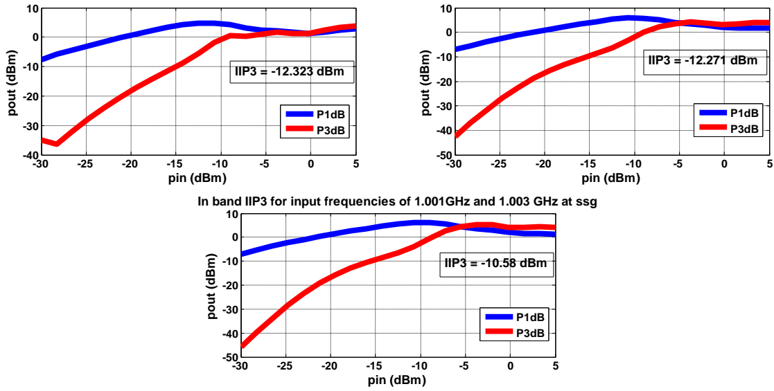
Fig.5.62 In band IIP3 for input frequencies of 1.001GHz and 1.003GHz at ssf, ssp and ssg
