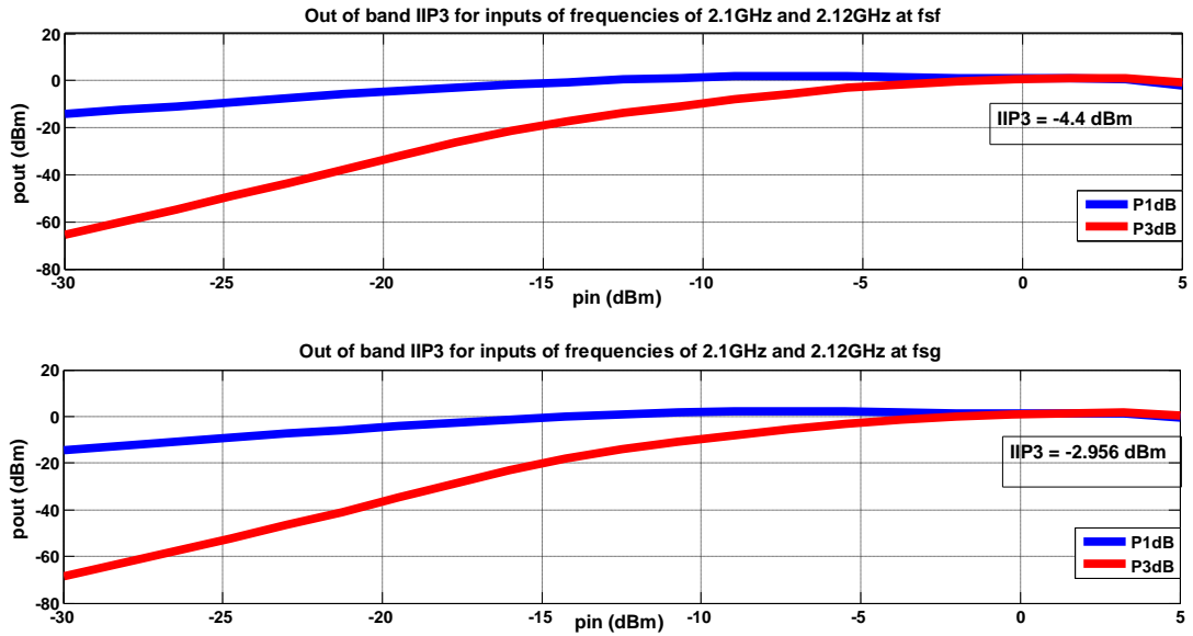
Fig. 5.30 Out-of-band IIP3 for input frequencies of 2.1GHz and 2.12GHz at fsf and fsg
