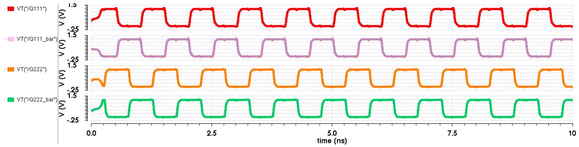
Fig. 4.23The quadrature 50% duty-cycle ( Q1\_MN , Q1\_bar\_MN , Q2\_MN and Q2\_bar\_MN )
