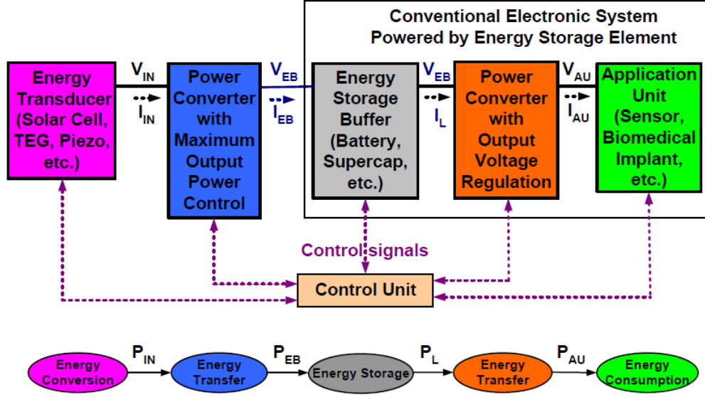
FIGURE 1.1: A typical block diagram of an energy harvesting system.[10]
