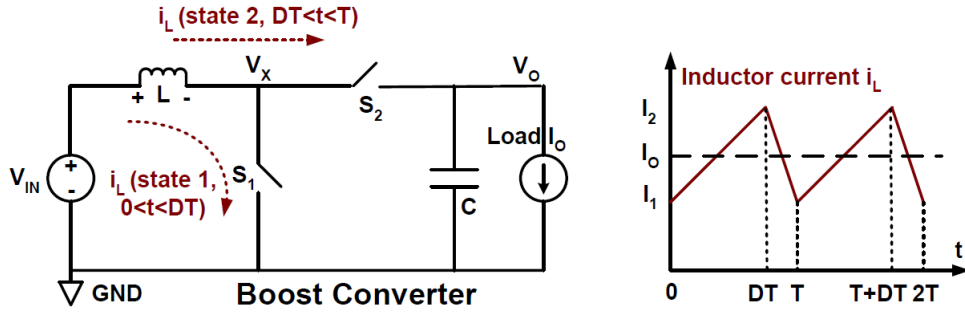
FIGURE 2.13: Schematic of a Boost Converter and Inductor Current Waveform [10]
