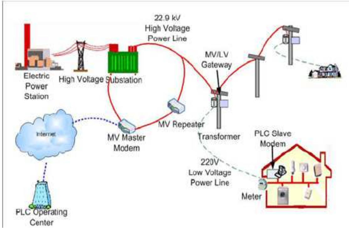
FIGURE 1.3: Overview of PLC Network Architecture with High voltage power line [5].
