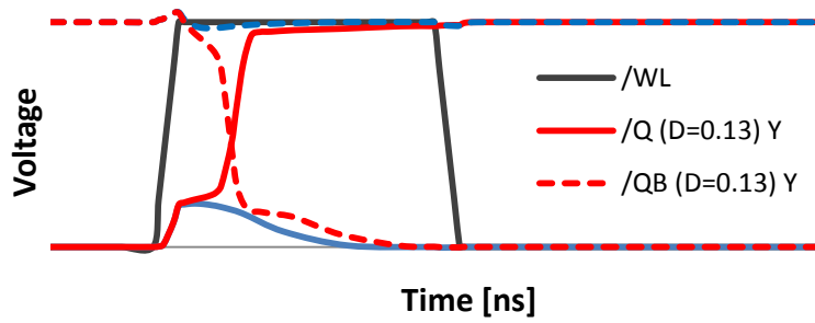
Internal Nodes self-capacitance (CQ)
