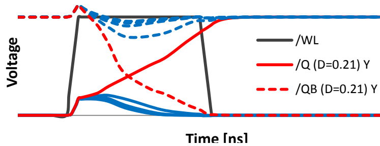
Overlap Capacitance (CWL-Q)
