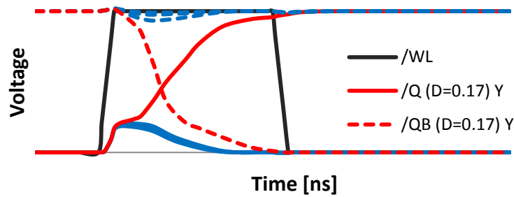
Internal Nodes Coupling capacitance [Miller Cap.] (CQ-QB)
