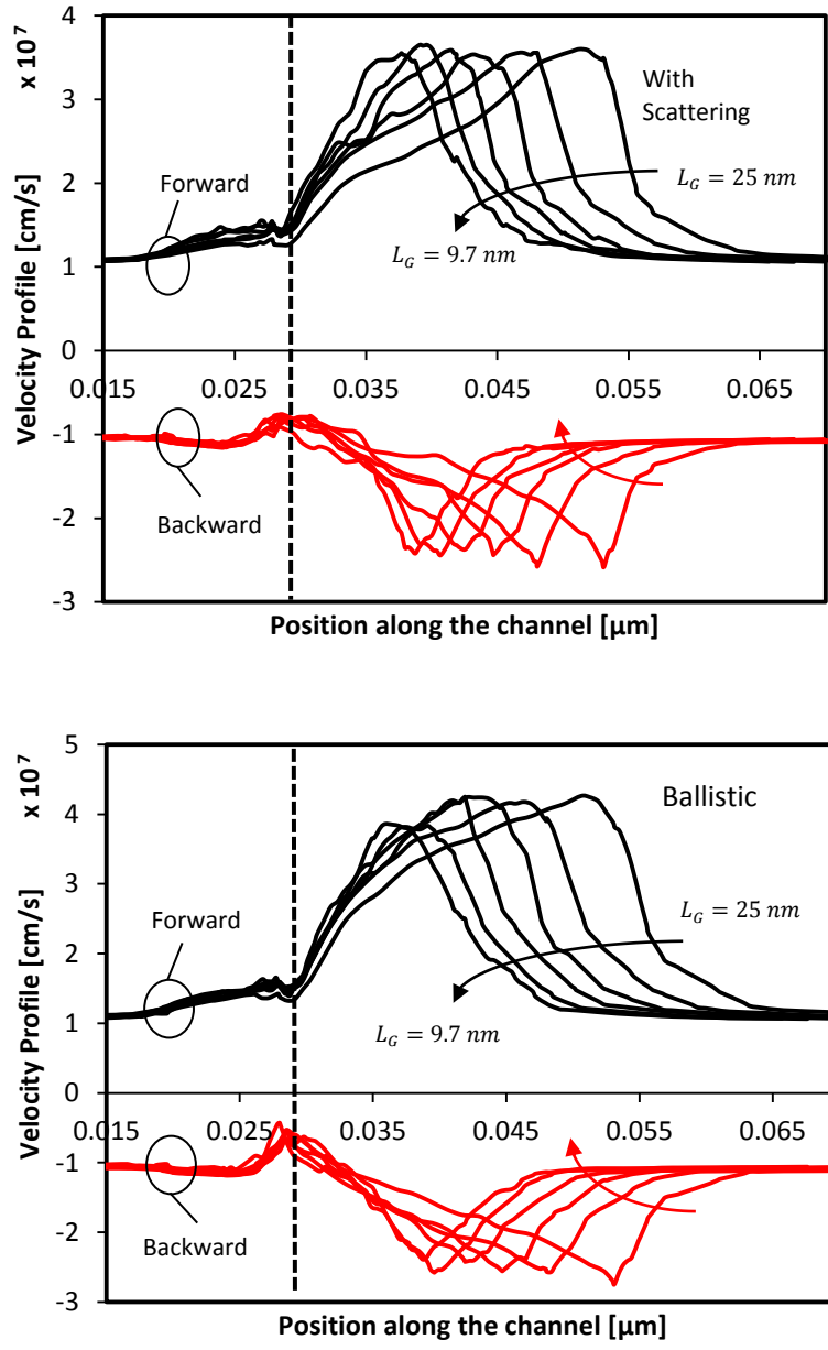
Figure 3-8: Forward and backward components of the electron velocity for Tri-gate FinFET 15 \text{ \AA}^\circ below the Si-SiO 2 interface at various channel lengths 25, 20, 16.7, 13.9, 11.6, 9.7 nm; a) For the Quasi-ballistic case (including scattering), b) For the ballistic case.
